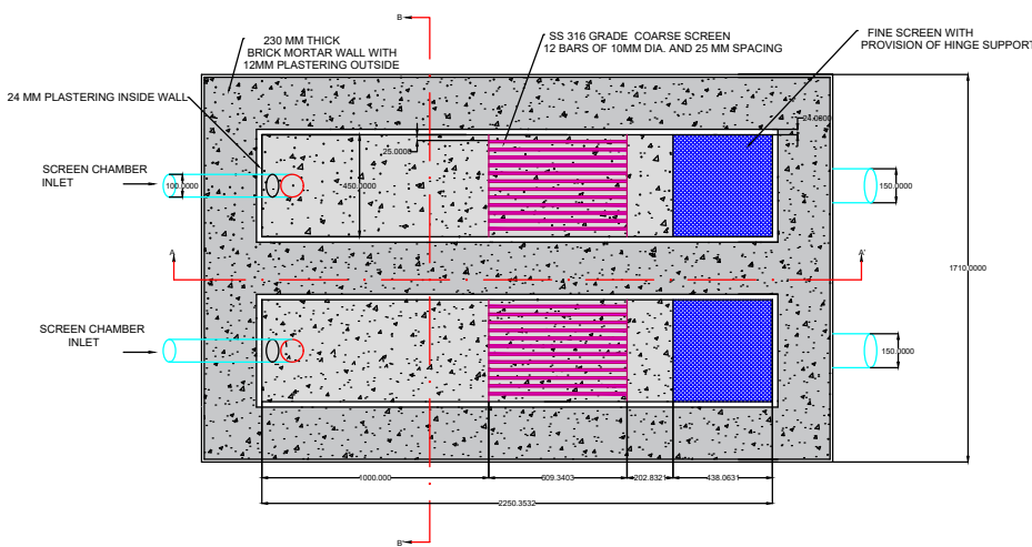
Figure 5: Plan and cross section for receiving chamber
