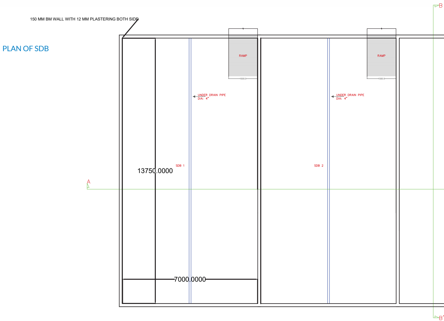
Figure 7: Plan and cross section of sludge drying beds for dewatered sludge
